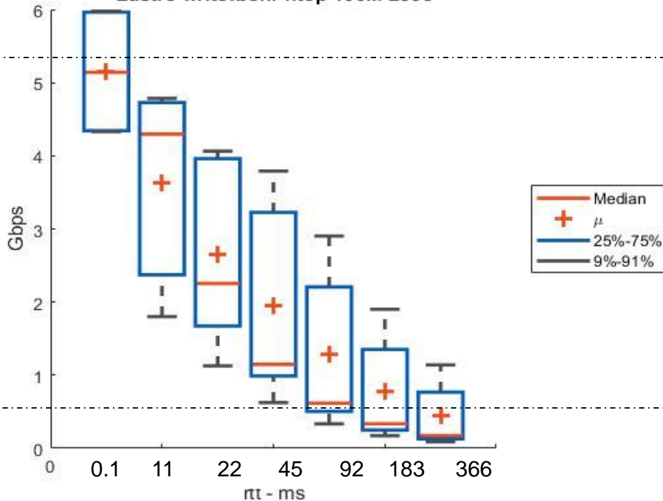
Lustre write:bohr htcp 100M 256c
